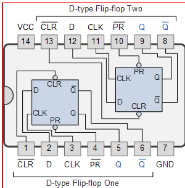
Dual D-Flip Flop (7474)
