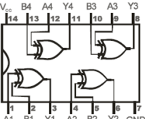
7486 Quad 2-Input XOR Gate
