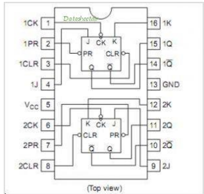
Dual JK- Flip-Flop (LS76A)
